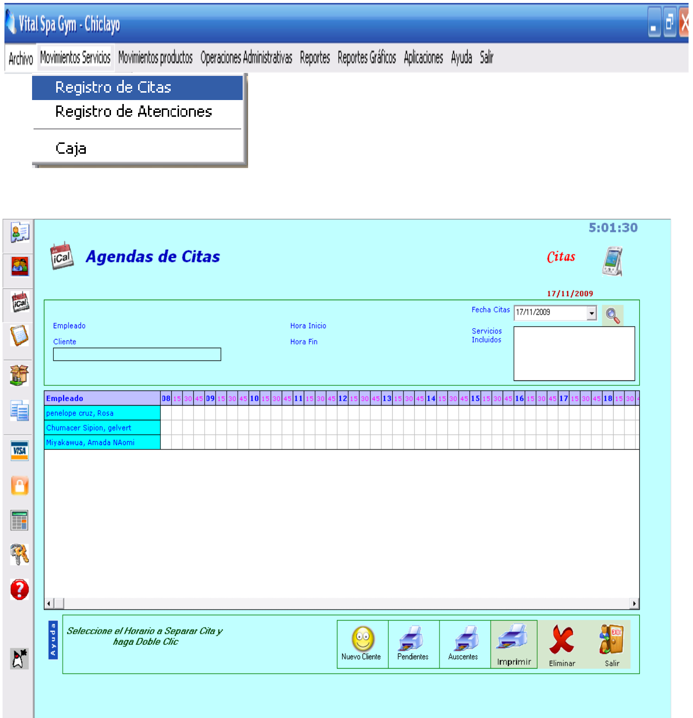
Fig.49: Formulario Citas
